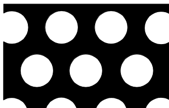
8φ 12P 40.0%
