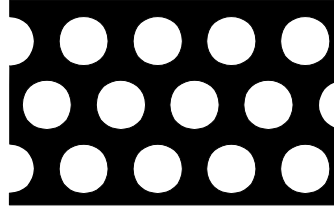
6φ 9P 40.0%
